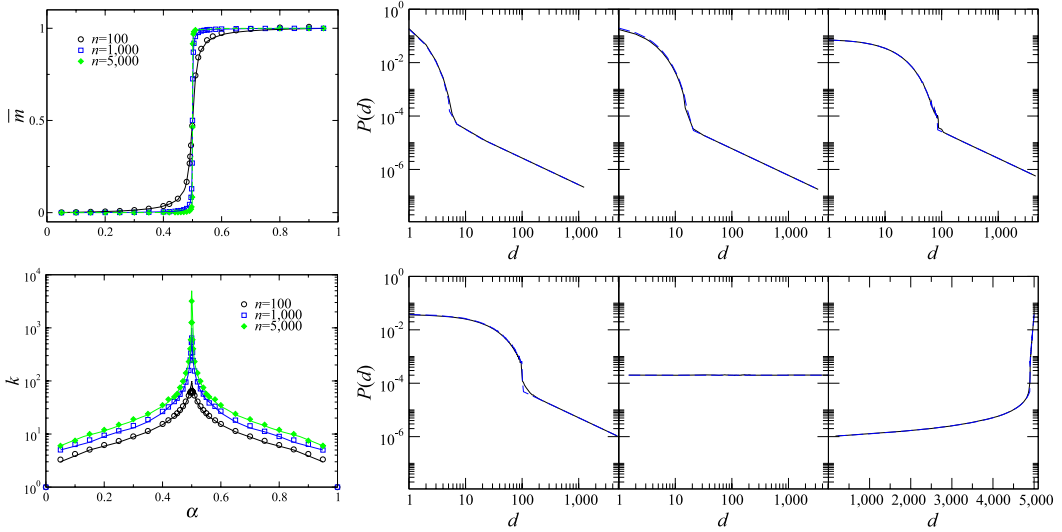
FIGURE 4. (Left) In the top panel we show the number \bar{m} of links m relative to the total number of possible links n(n - 1)/2 of the stationary network. The number of distinct degrees k = 2d^* , with d^* from (4), found in the stationary network for different values of \alpha are shown in the bottom panel. The figures display both the results obtained by recourse of numerical simulations (symbols) and by respecting theoretical predictions (lines) of the model. (Right) Degree distribution P(d) for different values of parameter \alpha and a network size n = 10,000 : \alpha = 0.2 (top-left plot), \alpha = 0.4 (top-center plot), \alpha = 0.48 (top-right plot), \alpha = 0.49 (bottom-left plot), \alpha = 0.5 (bottom-center plot), and \alpha = 0.52 (bottom-right plot). The solid line corresponds to the average of simulations, while the dashed line indicates the theoretical degree distribution from Proposition 5. The degrees have been binned to smooth the degree distribution.
