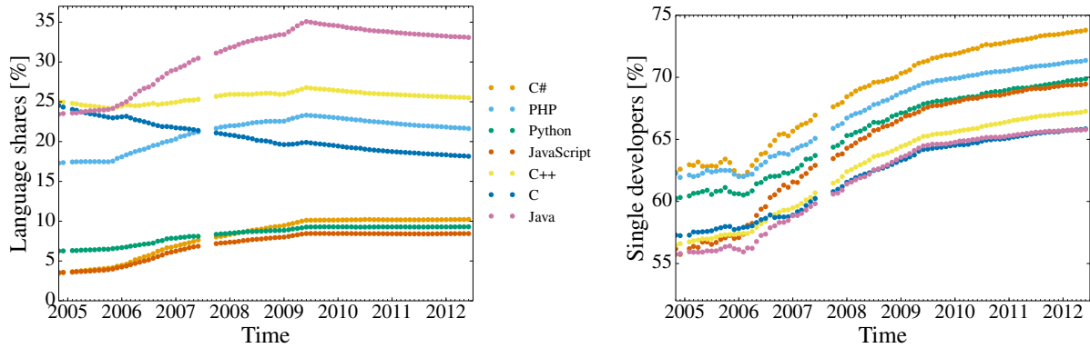
Figure 2: (left) Share of the 7 most popular programming languages (normalized to 100%) over time measured in months, for all projects with available information about programming languages. (right) Share of single-developer projects (normalized for each of the 7 most popular programming languages separately) over time measured in months.
