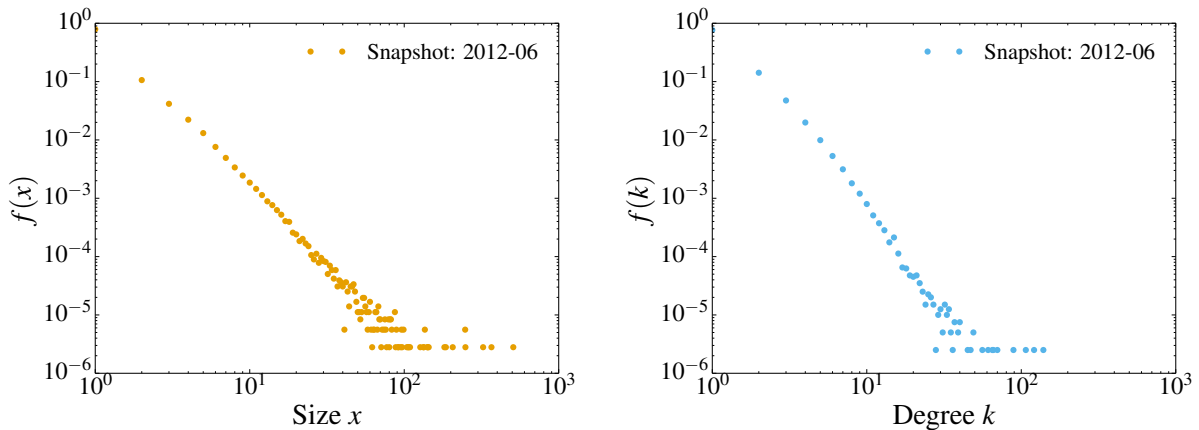
Figure 4: (left) Degree (size) distribution of projects (i.e., number of developers per project), f(x) , (right) Degree distribution of developers (i.e., number of projects a developer contributes to), f(k) , for the monthly snapshot of June 2012.
