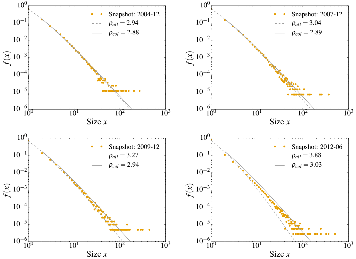
Figure 8: Project size distribution f(x) for different monthly snapshots. For each snapshot, a fit (dashed gray line) of the Yule-Simon distribution is plotted, for which the parameter \rho_{all} was numerically obtained. The goodness-of-fit test however rejects the hypothesis that the Yule-Simon distribution fits the empirical one for most of the snapshots. A second fit (solid gray line) of Yule-Simon distribution, for which the value for single-developer projects is taken as unknown, latent variable is also plotted, for which the same hypothesis cannot be rejected for the most of the snapshots.
