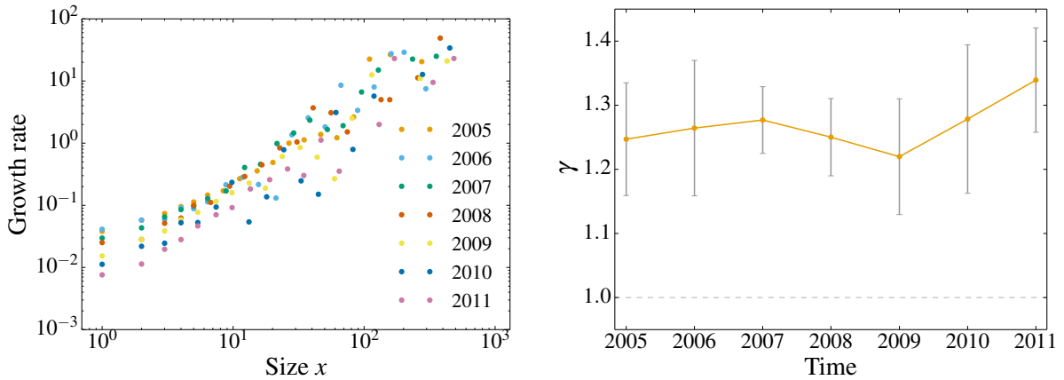
Figure 7: (left) Averaged annual growth rate \bar{g}(x) over project size x (measured by the number of developers) for each year separately. (right) Exponent \gamma , Eq. (3) for each year, where error bars indicate the standard error.
