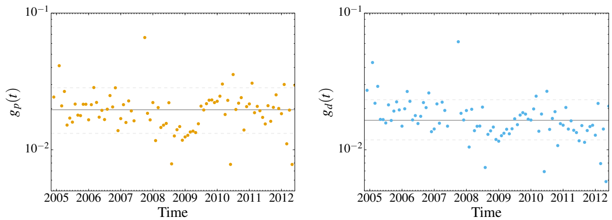
Figure 6: Relative monthly entry rate of projects, g_p(t) ( left ), and of developers, g_d(t) ( right ). The horizontal lines represent the median of all the values in the time series (solid line) and the dashed lines, 10% and 90% quantiles. The values read for g_p : 10%: 0.0131 , median: 0.0196, 90%: 0.0284, and for g_d : 10%: 0.0118, median: 0.0164, 90%: 0.0232
