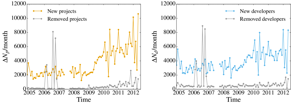
Figure 5: (left) Number of new projects (yellow) and removed projects (grey) per month. (right) Number of new developers (blue) and removed developers (grey) per month.
