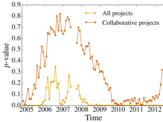
Figure 9: p -values for the goodness-of-fit test [1] of the Yule-Simon distribution and the empirical size distribution for each monthly snapshot. Collaborative projects refers to the project size distribution with corrected value for the single-developer projects. We observe that the Yule-Simon distribution is a plausible candidate for the size distribution of all projects only for certain periods of time, while for the corrected empirical distribution it is a plausible candidate for most of the times, notably from the late 2005 to the late 2009.
